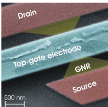
Electron micrograph of a bilayer graphene FET.
